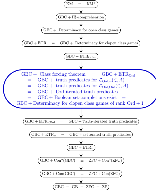
FIGURE 1. A hierarchy of theories between \text{GBC} and \text{KM} by consistency strength ( \equiv means equiconsistent)
